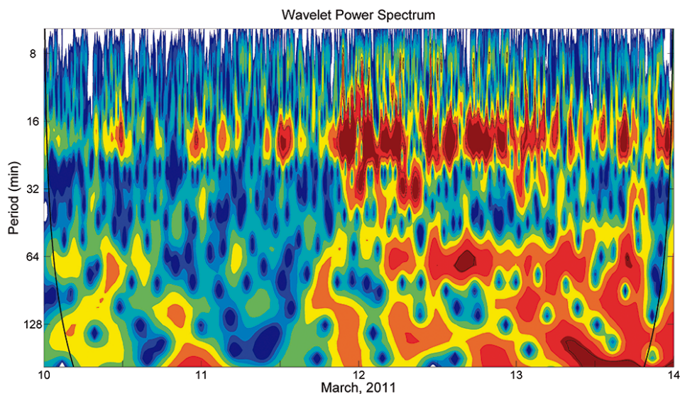
Figure 3 – The wavelet analysis showing the presence of the Tohoku tsunami waves in the sea level oscillations at Arraial do Cabo from March, 12 to March, 14.
