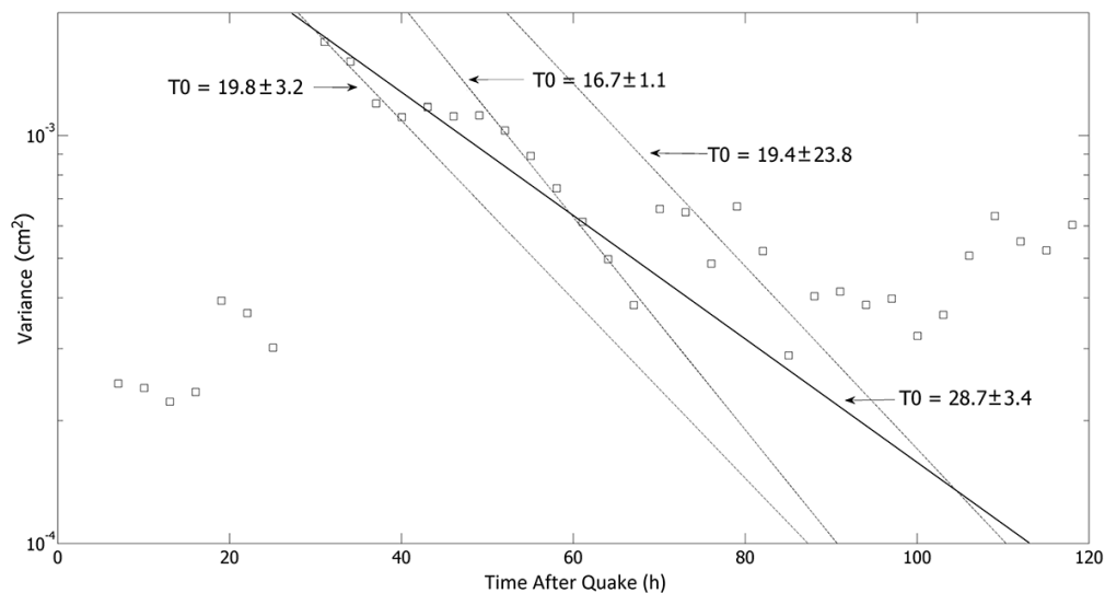
Figure 2 – Energy decay of the Japan tsunami recorded at Arraial do Cabo, showing the sea level variance changes with time. The secondary peaks of the variance are apparently associated with the wave trains reflected from the coasts of Africa and Antarctica.
