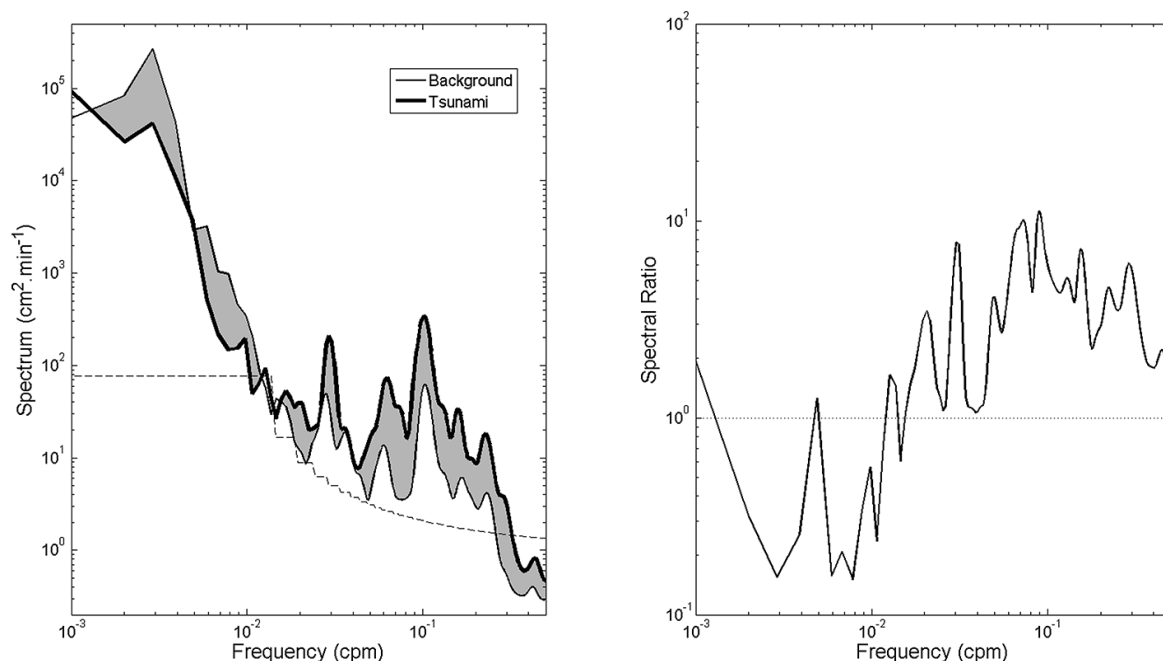
Figure 4 – Background (thin line) and tsunami (thick line) spectra estimated from the record of the Arraial do Cabo tide gauge (left panel). Spectral ratio (right panel) shows that the energy of tsunami was larger than the background in all frequencies above 0.0125 cpm.
